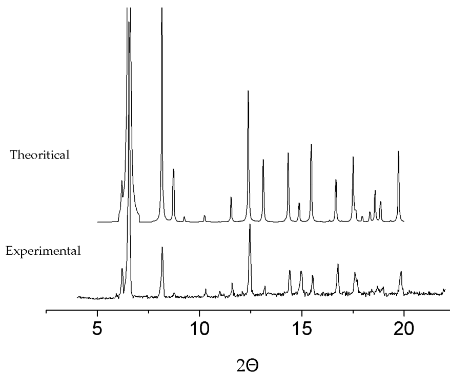
ESI 1 Powder XRD patterns for \text{Ti}_{16}\text{O}_{16}(\text{OCH}_2\text{CH}_3)_{26}(\text{OCH}_2\text{CCl}_3)_6 ( \lambda = 1.5417 \text{ \AA} ).
