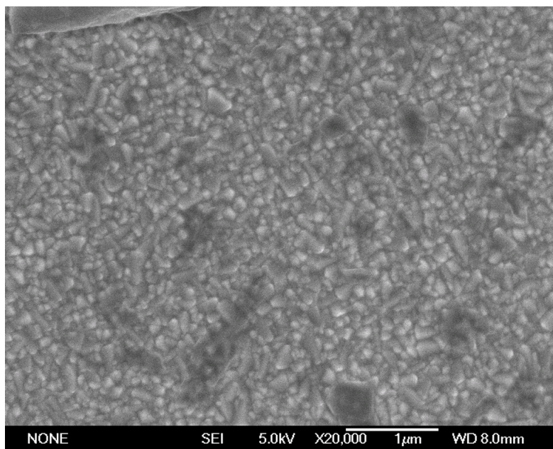
Figure S1. SEM micrograph of Fe-TsO coated films (20 wt%)
