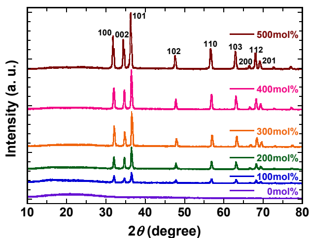
Fig. S1 XRD patterns of ZnO-NP/PI blend hybrid films: Blend-0 – 500 .
