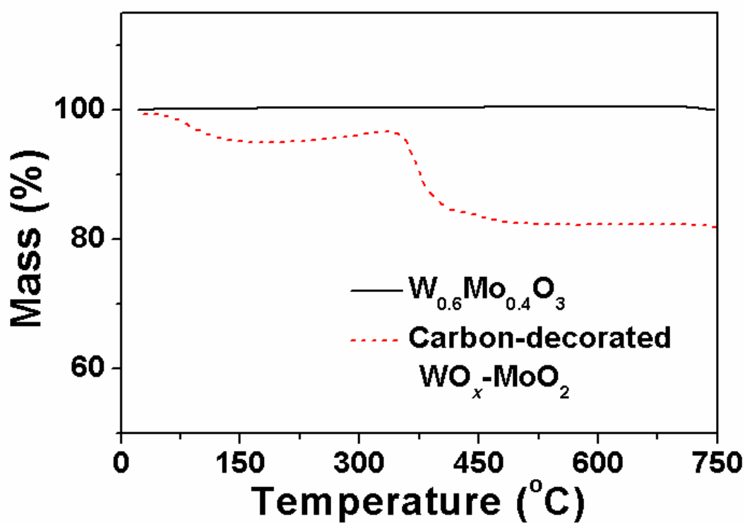
Fig. S1 TGA plots of W_{0.4}Mo_{0.6}O_3 and carbon-decorated WO_x-MoO_2 nanorod samples.
