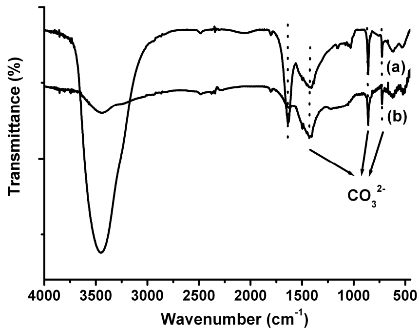
Fig. S1 The FT-IR spectra of the as-prepared precursors obtained in the presence of \beta -cyclodextrin (a) and fructose (b).
