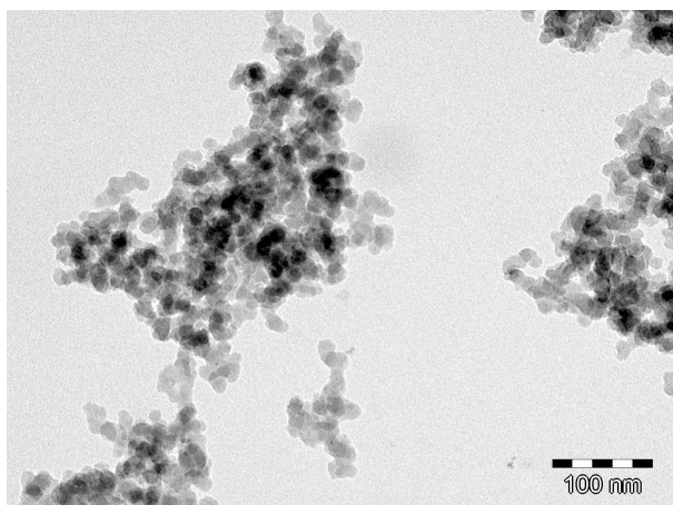
Fig. S1: TEM image of Al/SiO 2 .
