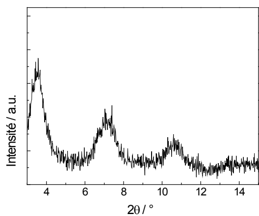
Fig. S3: Powder XRD pattern of the sample AS10 (23.8 OPA/nm 2 ).
