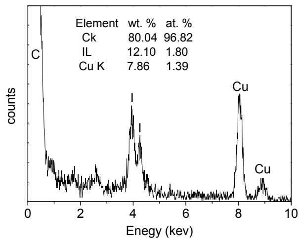
Figure S2 EDS micro-analysis of iodine-filled carbon nanocages indicates they are comprised primarily of carbon (C) and iodine (I), indicating iodine is encapsulated in carbon nanocages.
