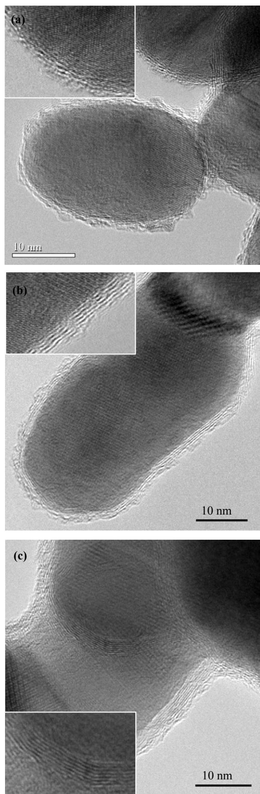
Figure S1. Enlarged versions of HRTEM images shown in Figure 2 for CNC A (a), CNC B (b) and CNC C (c) from the mixture of pyridine and iron pentacarbonyl with a volume ratio of 1:100, 1:10, and 1:1, respectively.
