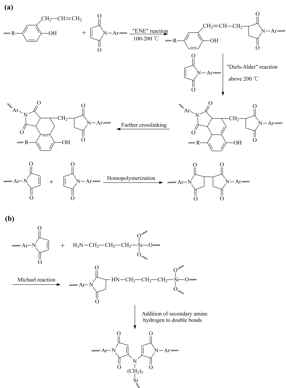
Scheme 1S The chemical reactions among BDM, DBA and Am-HPSi
