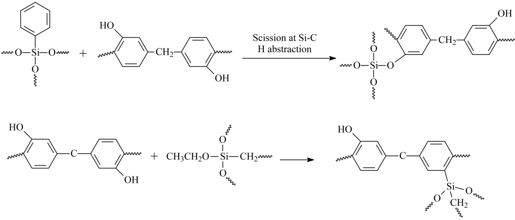
Scheme 2S The cross-linking reactions between Am-HPSi and BDM/DBA resin
