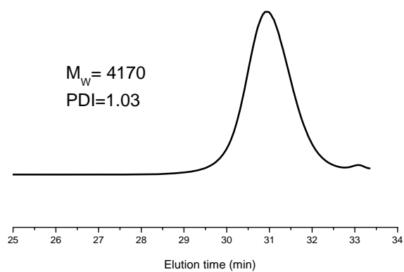
Figure S7. GPC of BS-PSQ
