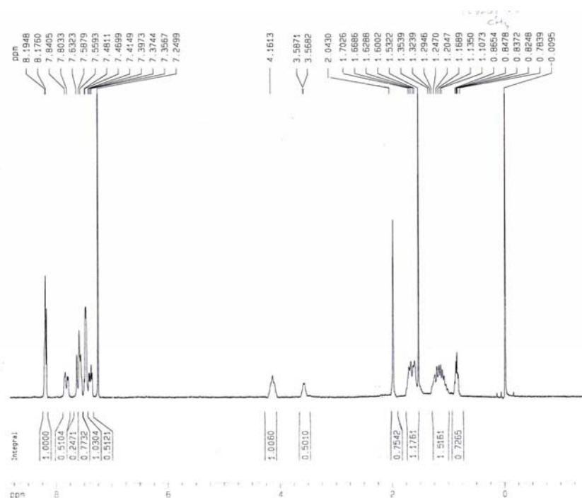
Figure S4. ^1\text{H} NMR of M_2
