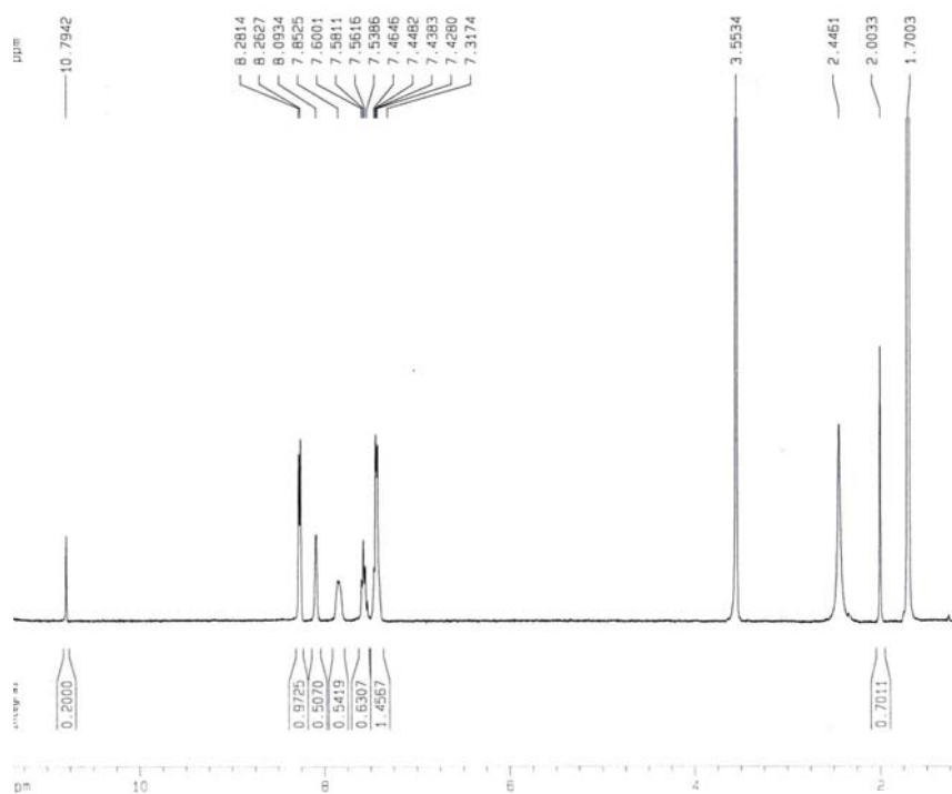
Figure S2. ^1\text{H} NMR of M_1
