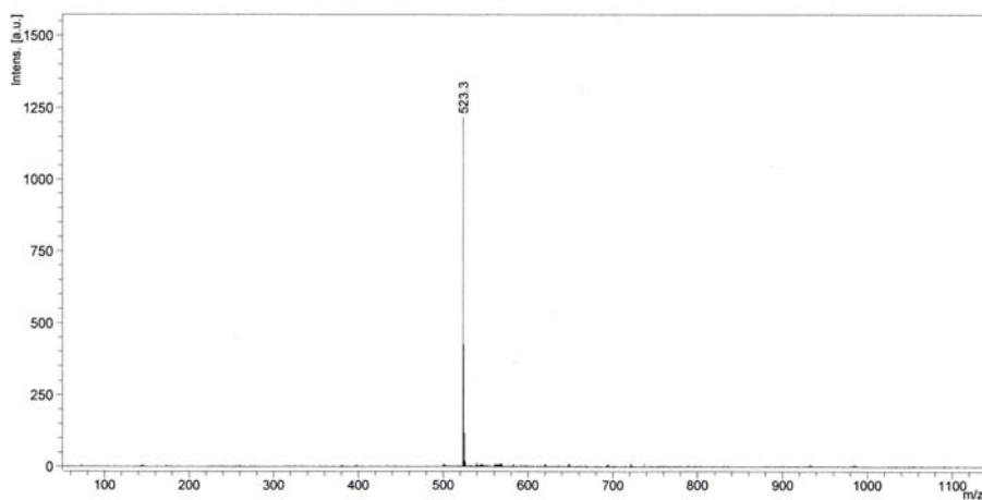
Figure S1. MALDI-TOF MS of M_1
