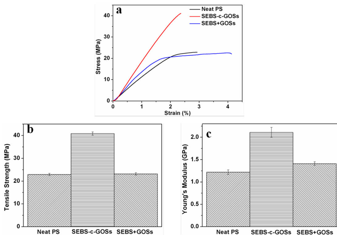
Fig. S6 (a) Representative stress-strain curves and (b), (c) mechanical data of neat PS, PS/2.0 wt% SEBS-c-GOS composite (SEBS-c-GOSs) and PS filled with 0.7 wt% SEBS and 1.3 wt% GOSs (SEBS+GOSs).
