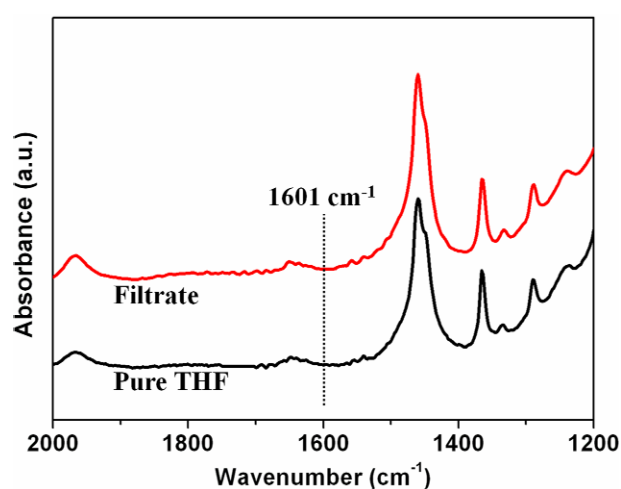
Fig. S1 FTIR spectra of pure THF and filtrate.
