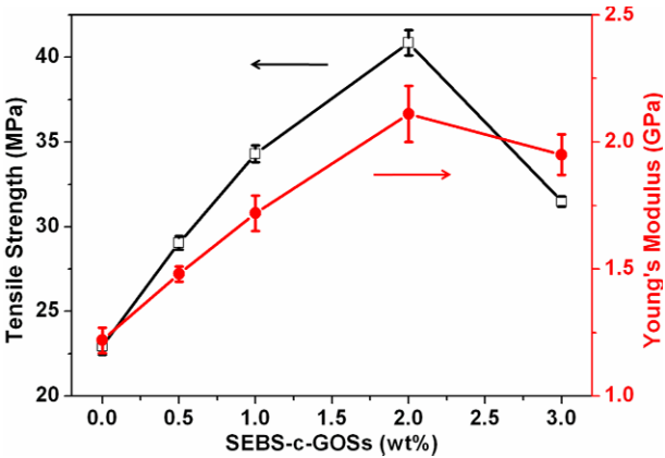
Fig. S5 Relationships of tensile strength and Young's modulus with SEBS-c-GOS concentration.
