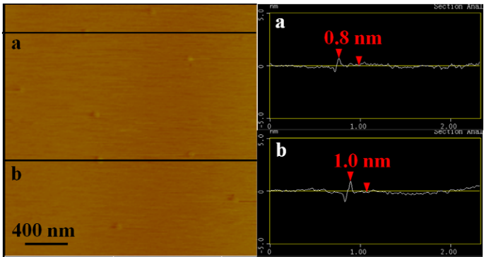
Fig. S4 AFM image (left) and height profiles (right) of chloroacetylated GOSs.
