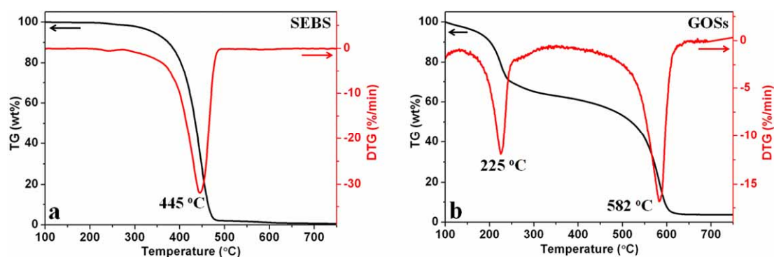
Fig. S2 TGA and DTG traces for (a) SEBS and (b) GOSs.
