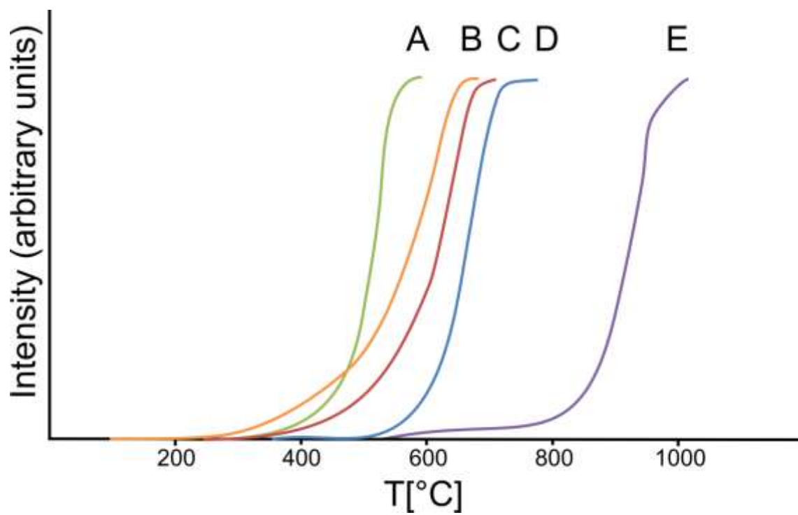
Figure A1: Temperature programmed oxidation of methane performed with A) pure ceria, B) A100-C30, C) A100-C10, D) A100-C05 and E) the empty sample cell.
