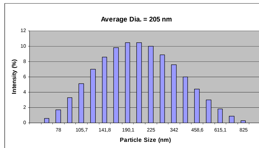
Histogram of size distribution of CZTS nanocrystals
