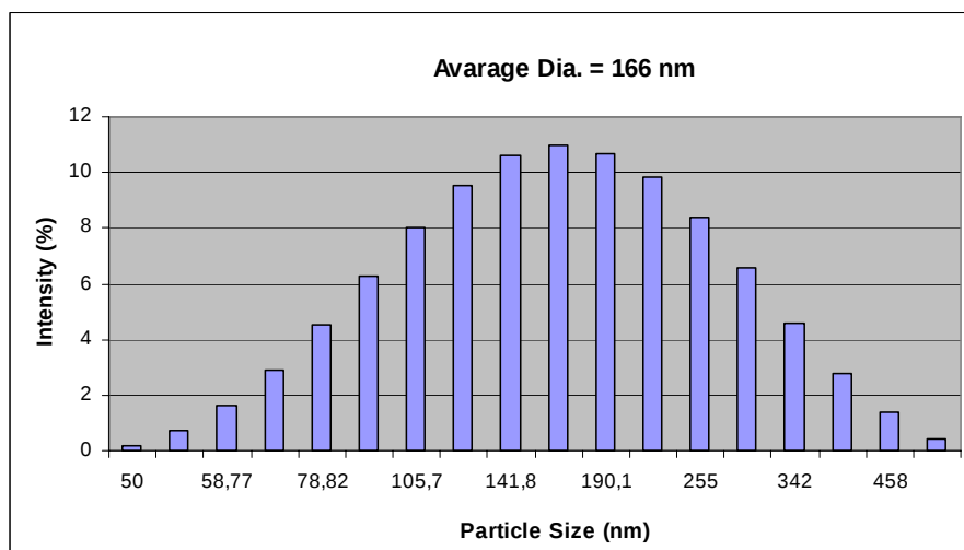
Histogram of size distribution of CCTS nanocrystals
