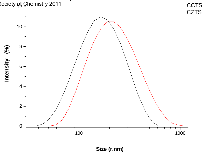
Size distribution by DLS ( log scale)
