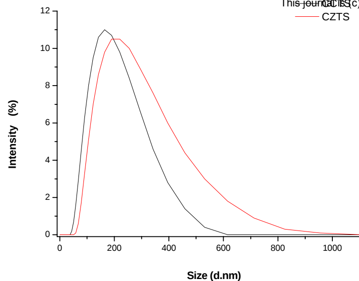
Size distribution by DLS
