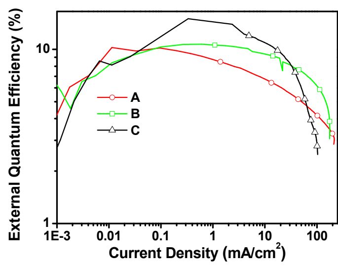
Figure S1. External quantum efficiencies versus current density curves of the devices.
