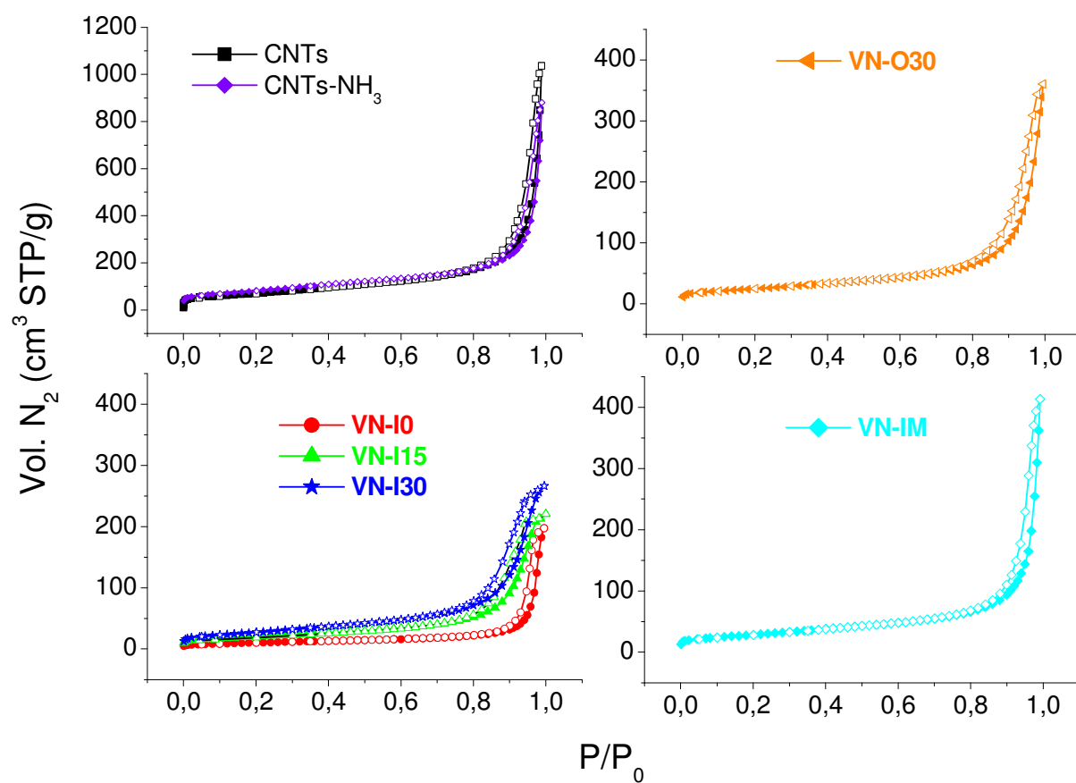
Fig 1 Nitrogen adsorption/desorption isotherms of CNTs, CNTs-NH 3 , VN, and VN/CNTs materials at 77 K (closed dot: adsorption and open dot: desorption).
