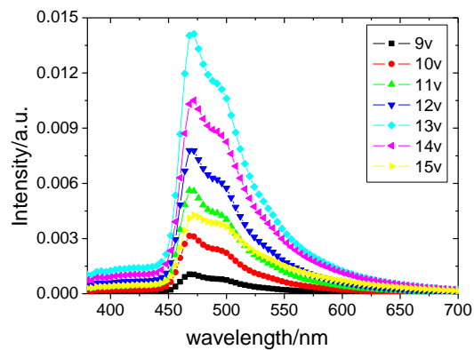
Figure S3. EL spectra with different voltages for device ITO:PEDT/PVK/ TP:FlrPic /TPBi/LiF:Al
