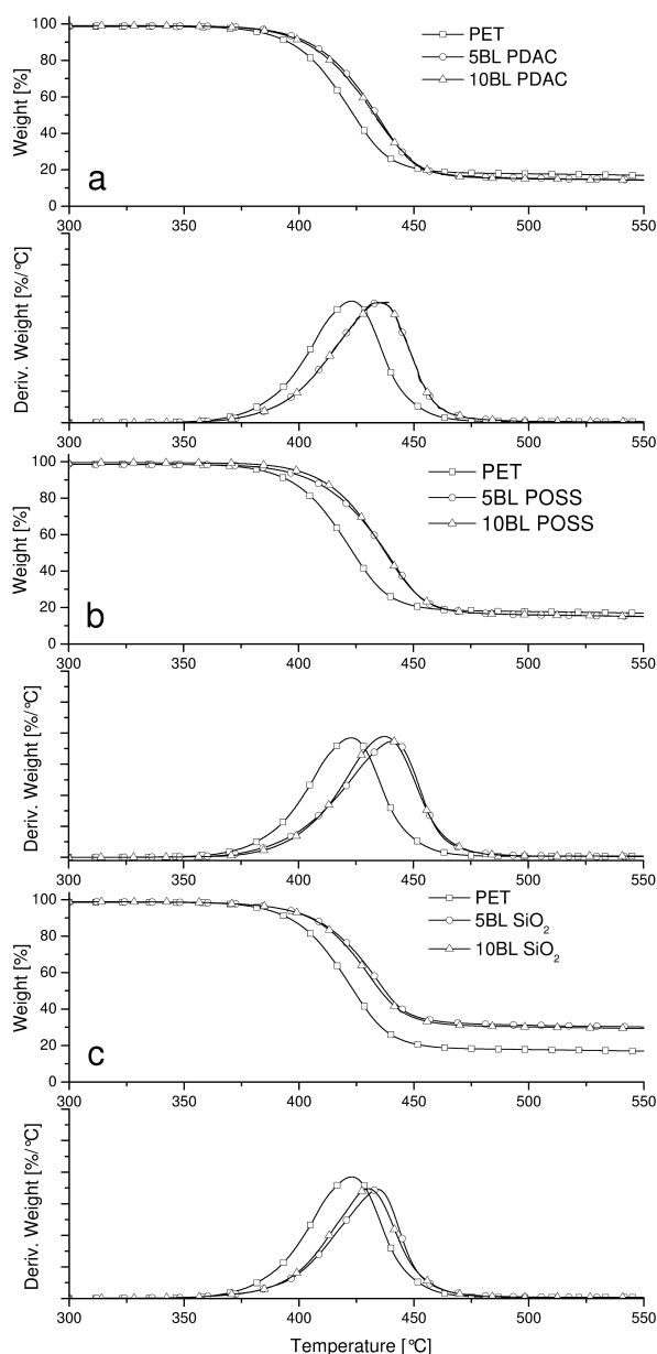
Figure S1. TG and dTG curves of neat PET, PDAC (a), POSS (b) and SiO 2 (c) treated fabrics in nitrogen.
