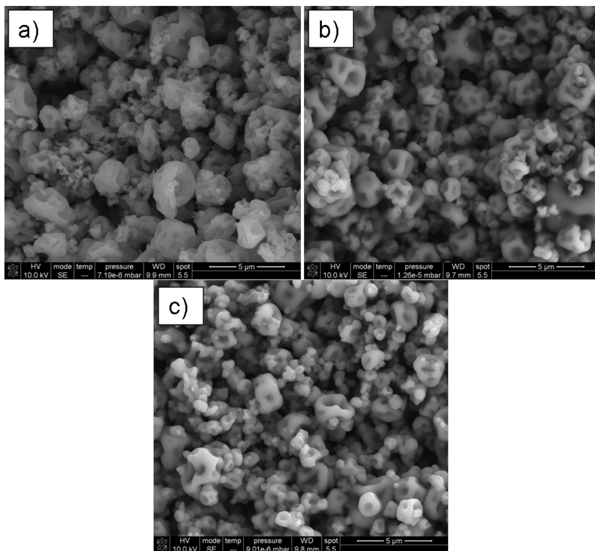
Fig. S1: SEM micrographs of a) Ti 1 -700, b) Ti 0.95 Nb 0.05 -700 and Ti 0.9 Nb 0.1 -700
