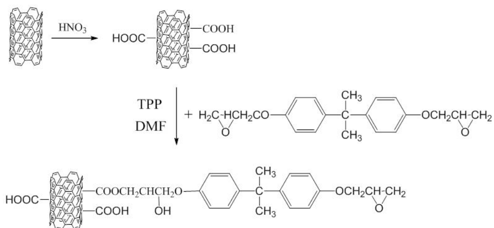
Scheme 1S The surface treatment of MCNTs
