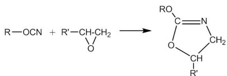
Scheme 2S The reaction between epoxide and -OCN groups
