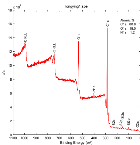
Figure S1. XPS spectra: wide region of GO (A), RFGO (B1) and RSGO (C); S 2p XPS spectra of RFGO (B2)
