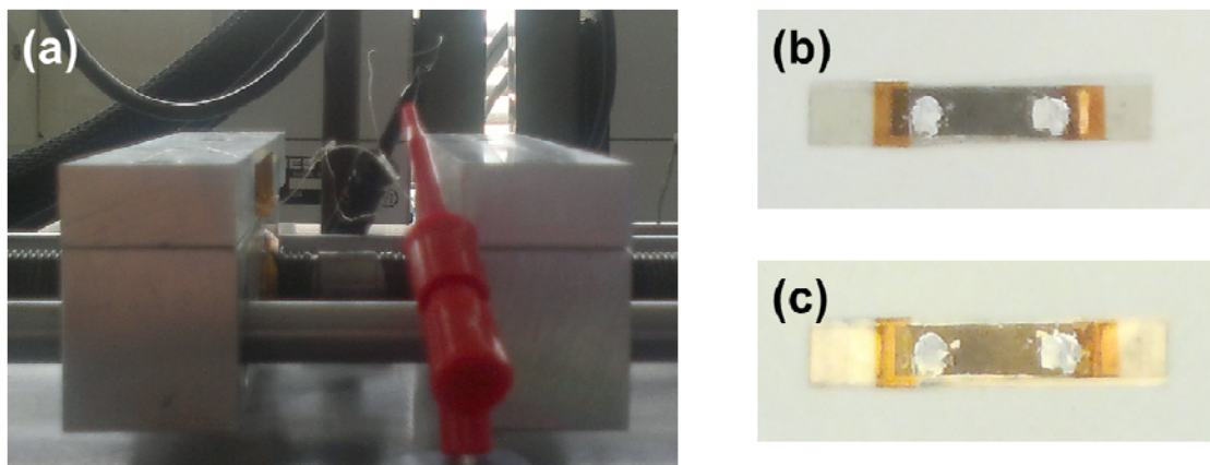
Figure 2: Physical stability of the SWNT/CNH composite. A strip of composite film was bent for 1000 cycles as shown in (a) while the conductivity was measured. (b) and (c) show photographs of the films before and after, no visible deterioration, in the structure of the film or the conductivity was observed.
