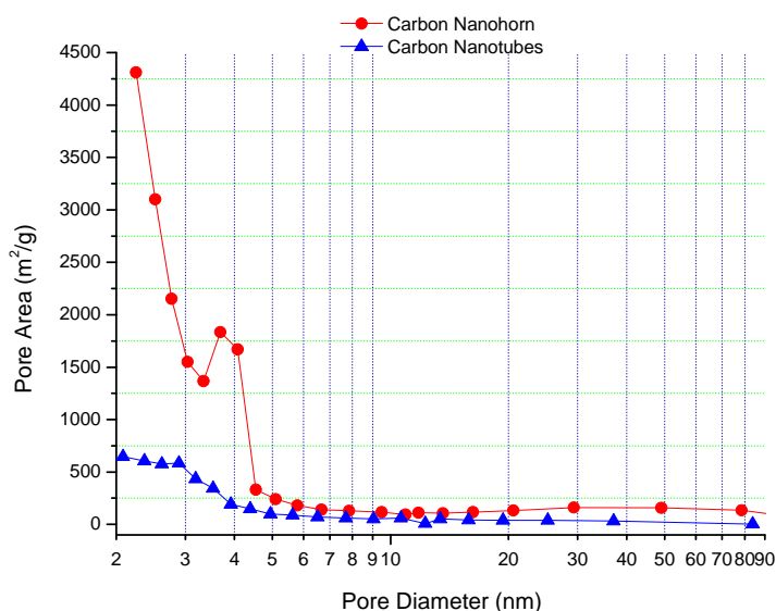
Figure 1: Barret-Joyner-Halenda (BJH) analysis of the CNTs and the CNH. It can be seen that a large part of the surface area enhancement comes from micropores (<2nm).
