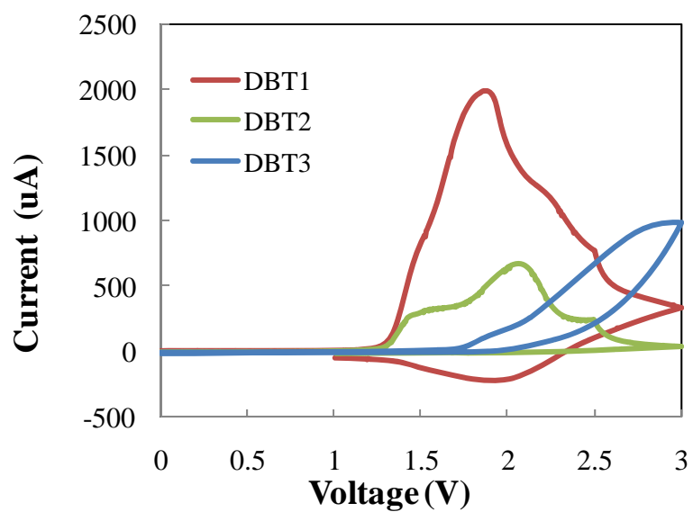
Figure S1 Cyclic voltammetry curves of DBT1, DBT2 and DBT3.
