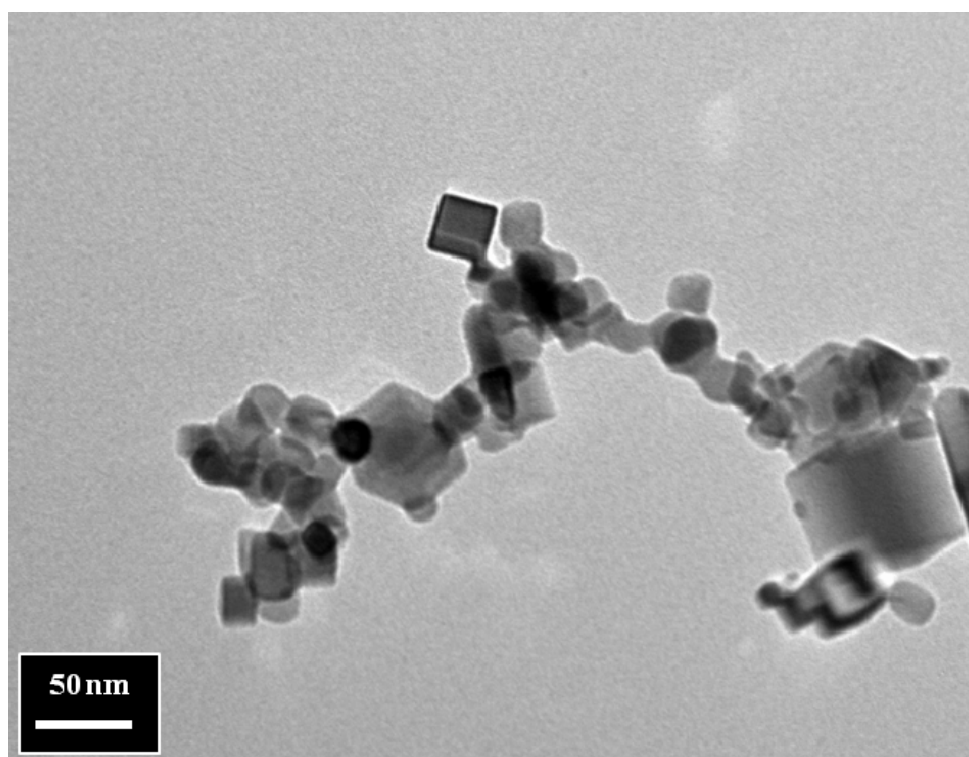
Figure S1 TEM image of TiN-NPs.
