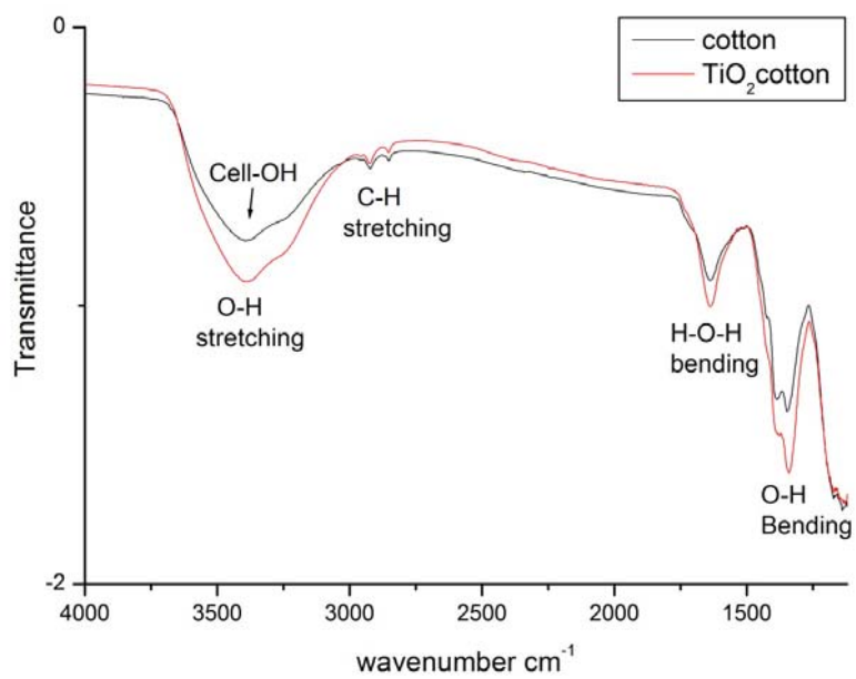
Fig S1. ATR-FTIR spectra for pristine cotton fabric and \text{TiO}_2 treated cotton fabric.
