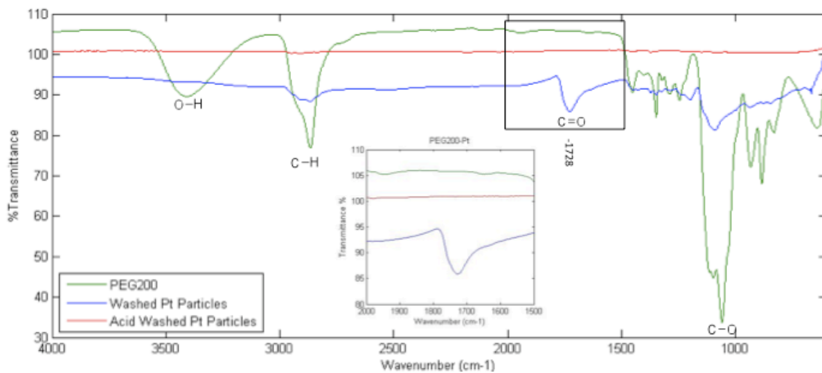
Figure S2. Normalized FTIR spectra of PEG200, washed PEG200 platinum and acid washed PEG200 platinum nanoparticles.
