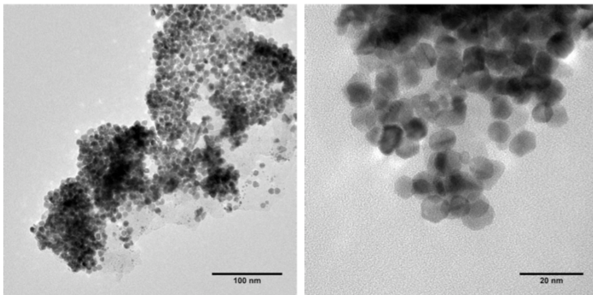
Figure S3. Low and high magnification TEM images of the PEG200 synthesized platinum particles after washing with 0.1M H 2 SO 4 .
