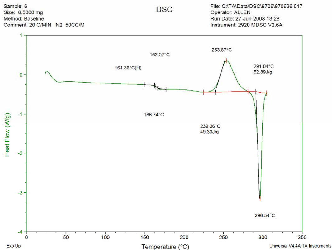
Figure S-1: The DSC plot of CMesB .
