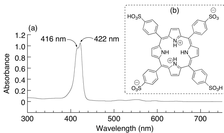
Fig. S1 (a) UV-Vis spectrum of TPPS in methanol (concentration = 4 \mu\text{mol/L} ) and (b) chemical structure of TPPS.
