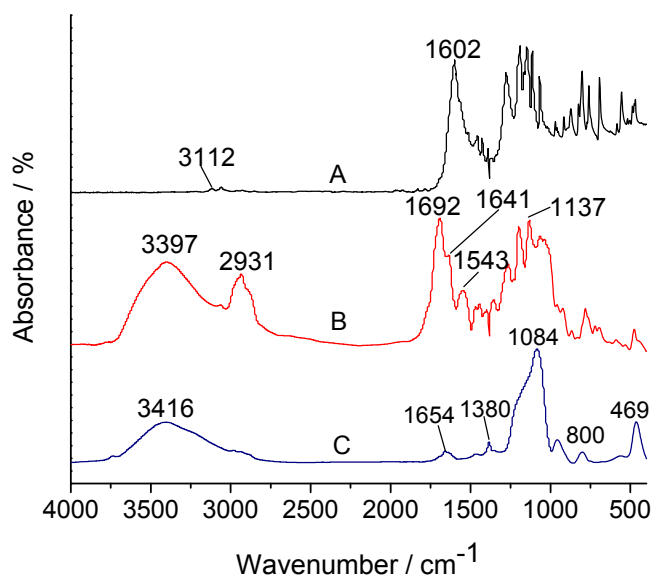
Figure S1. FTIR spectra of NTA(A), NTA-Si (B) and NTA-functionalized mesoporous hybrid material NTA-S15 (C).
