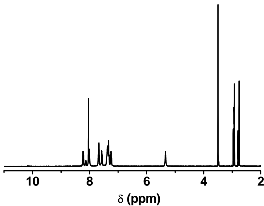
Fig. S2 Original 1 H NMR spectrum of 6F-BAHP-PC PI
