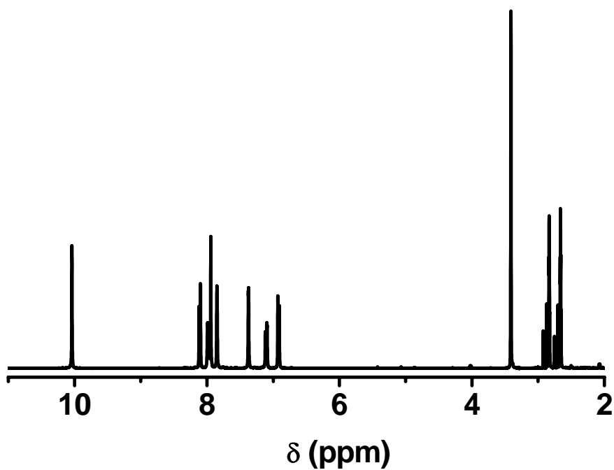
Fig. S1 Original 1 H NMR spectrum of 6F-BAHP PI
