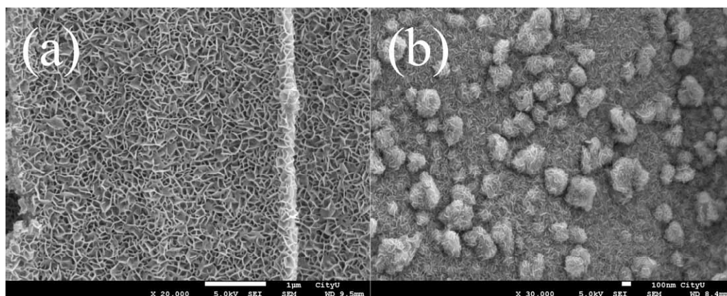
Fig. S1 The morphology of the active materials after 2000 cycles measurements: (a) Ni(OH) 2 on the side-wall; (b) Co(OH) 2 on the side wall.
