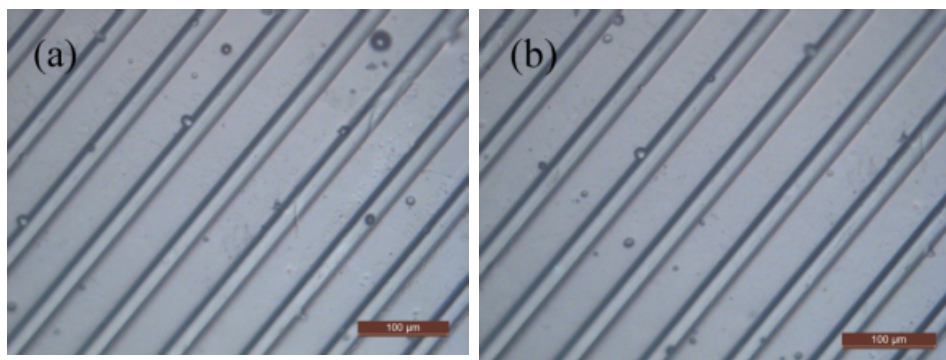
Fig. S2 Optical image of PDMS before (a) and after (b) imprinting process
