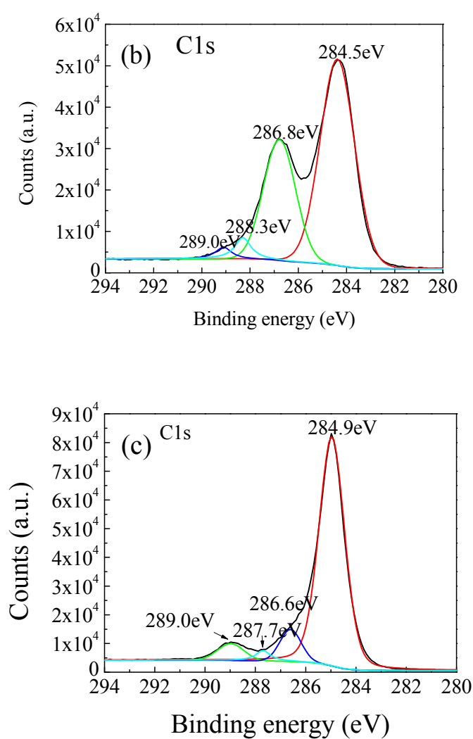
Fig. S2 (a) XPS survey of as-made GO and rGO, (b) C1s spectra of GO, (c) C1s spectra of rGO
