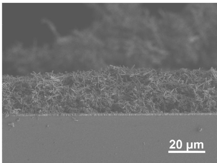
Figure s2: Cross-section view SEM image of the nanorod film.
