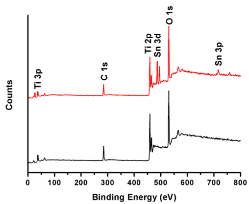
Fig. S1. XPS survey spectra of the Sn-doped (upper) and undoped (lower) samples showing the elements detected.
