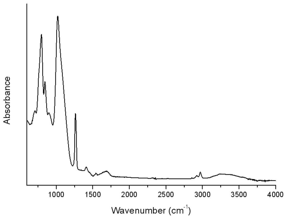
Fig. 6 FTIR spectra of the hybrid coating produced from hexamethyldisiloxane and the luminescent coordination polymer.
