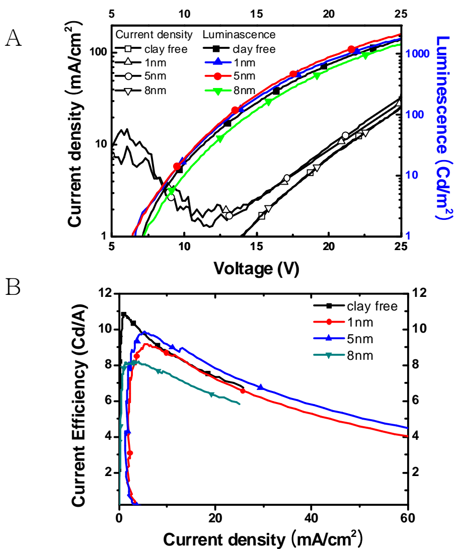
Figure S1. Initial Current density-Voltage-Luminescence curves (a) and Current efficiency-Current density curves (b).
