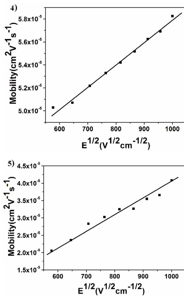
Figure S3. Electron mobilities of compounds 1-5.
