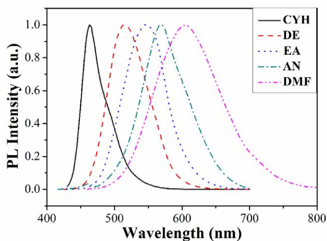
Figure S1. PL spectra of 5 in different solvents in room temperature. CYH=Cyclohexane, DE=Diethyl ether, EA=Ethyl acetate, AN=Acetonitrile, DMF=Dimethyl formamide.
