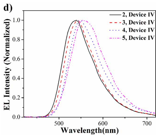
Figure S4. EL spectra of Devices. a): Device I; b): Device II; c): Device III; d): Device IV.
