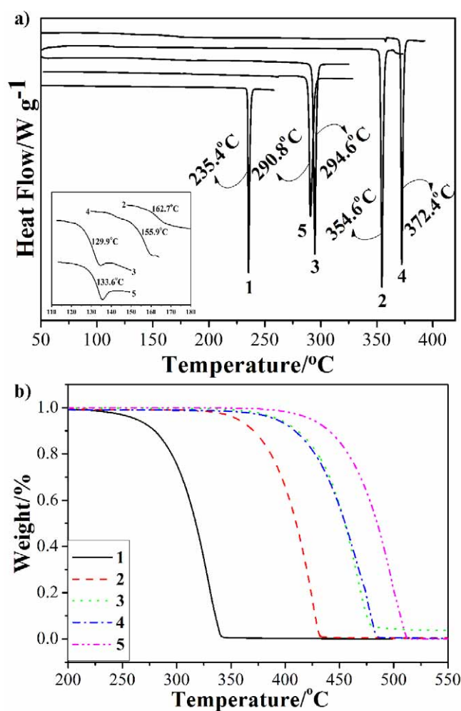
Figure S2. a): DSC data of 1-5. b): TGA data of 1-5.
