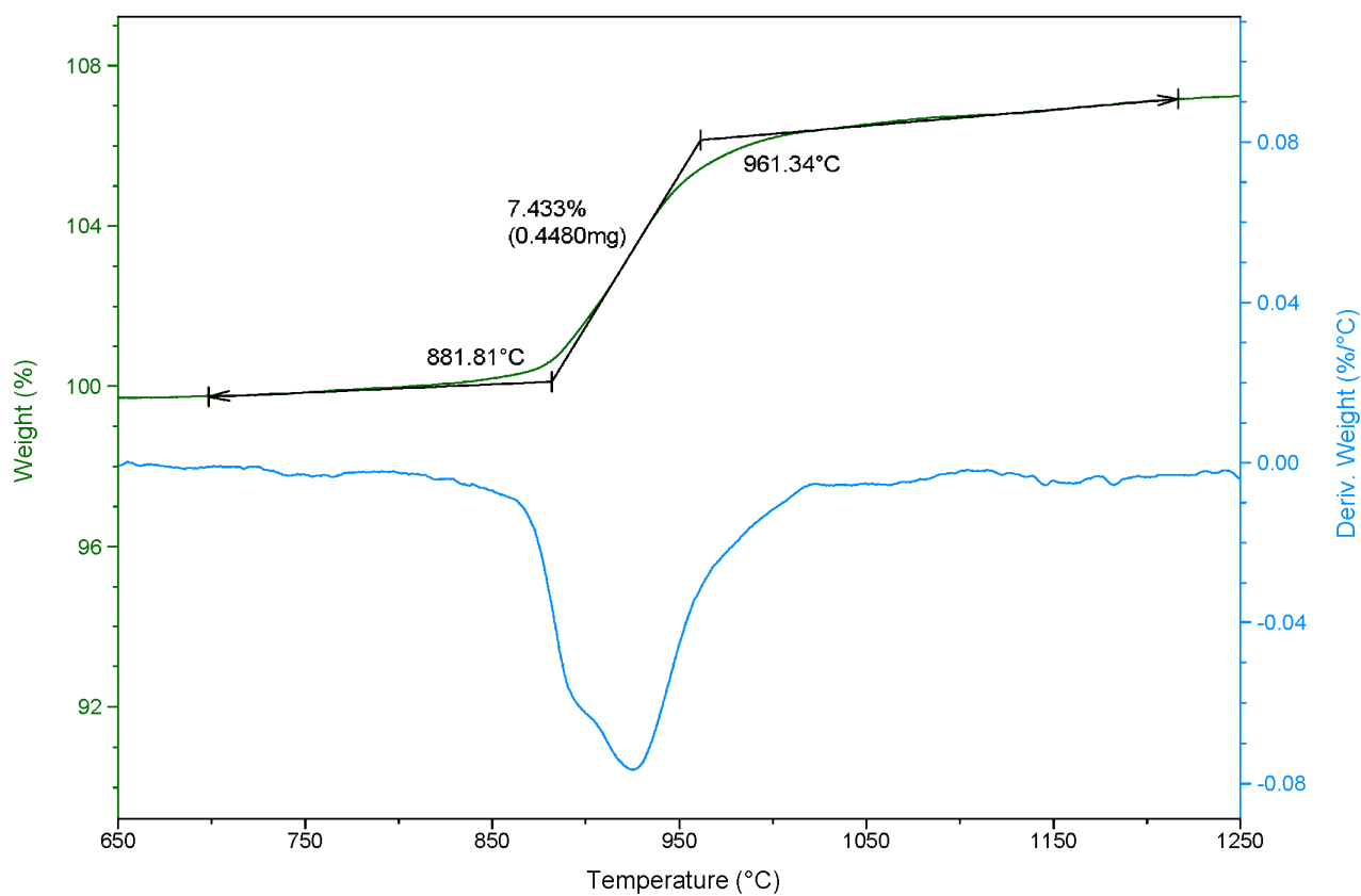
Fig.2 Thermogravimetric Analysis
