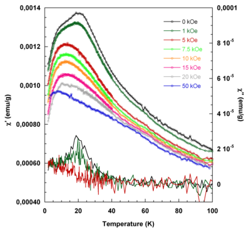
Figure S1. Effect of a superimposed dc field on \chi' in the low temperature region.
