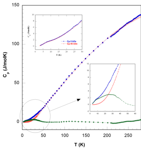
Figure S2. Specific heat measurements of oxidized material between 1.8 and 300 K.
