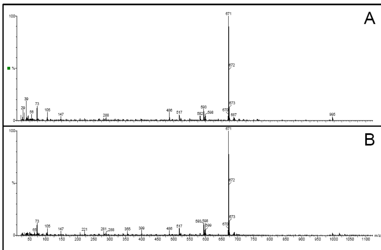
Figure S1: ESI-MS spectra of : A) CoTPP after deposition by GDS technique; B) pristine CoTPP powder.
