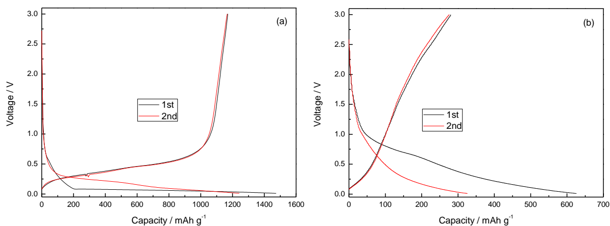
Figure S1. Voltage profiles of the pristine Si (a) and pure graphene (b) electrodes at a current density of 300 mA
