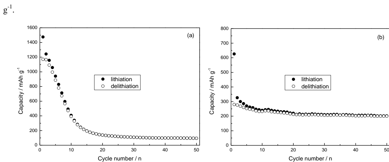
Figure S2. Cycling performance of the pristine Si (a) and pure graphene (b) electrodes at a current density of 300 mA g -1 .
