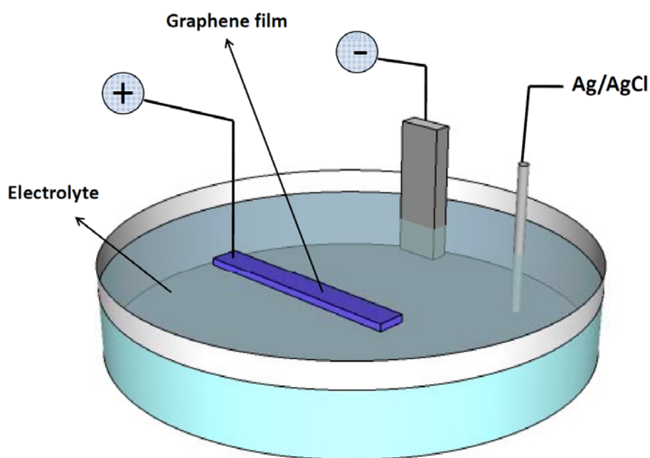
Fig. S1 Experimental setup to produce a bilayer structure of PPy(ClO 4 - ) and graphene film by a floating polymerization method.
