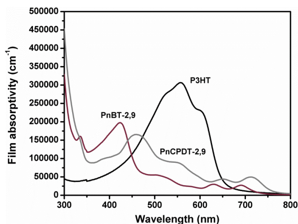
Figure S2. Film absorptivity of PnBT-2,9 and PnCPDT-2,9 as compared to P3HT, indicating the pentacene-containing polymers' lower absorptivity. PnCPDT-2,9 absorbs more intensely in the visible wavelengths than PnBT-2,9 .
