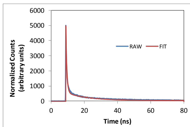
Figure S1. PL decay curves ( \lambda_{\text{ex}}=350 nm) of CdS 2.7 at RT
