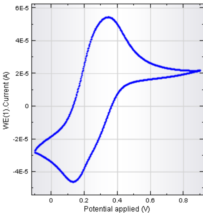
Cyclic voltammogram of polymer 4 , 1mg/ml, 0.1 M NaCl
