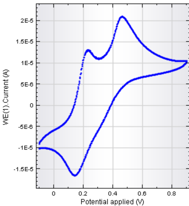
Cyclic voltammogram of polymer 4 , 1mg/ml, 0.1 M NaCl
