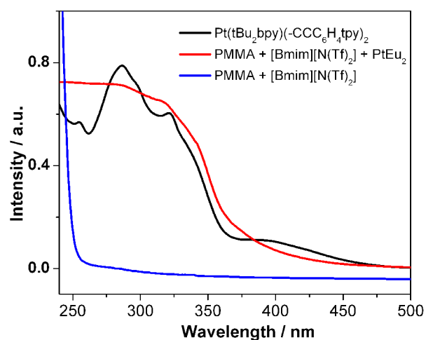
Figure S1. UV-Vis electronic absorption spectra of (Bu t 2 bpy)Pt(C≡CC 6 H 4 tpy) and ionogels.
