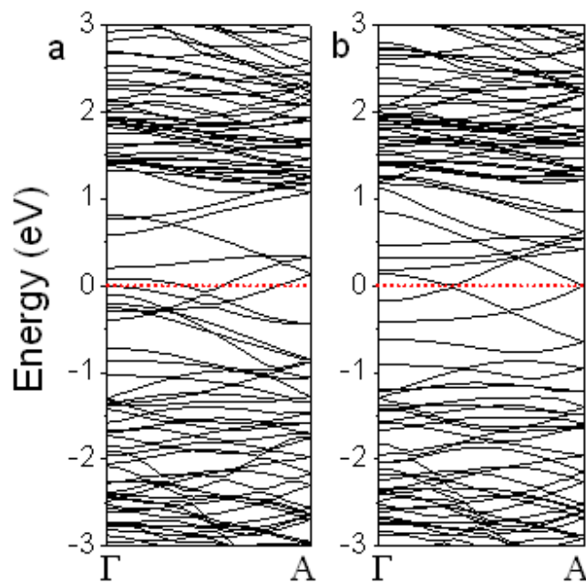
S-4, The calculated band structures of zz-MoS 2 -NR-Mo-u: (a) spin-up and (b) spin-down.
