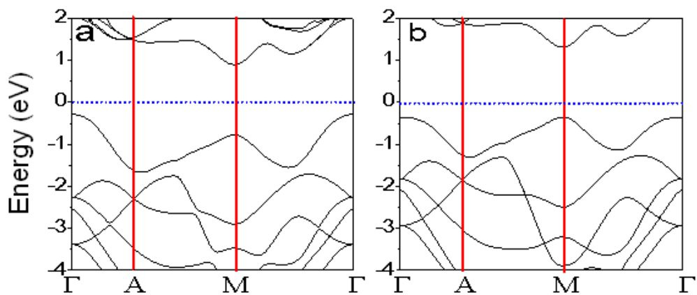
S-1, The calculated band structures of MoS 2 : (a) bulk and (b) monolayer.
