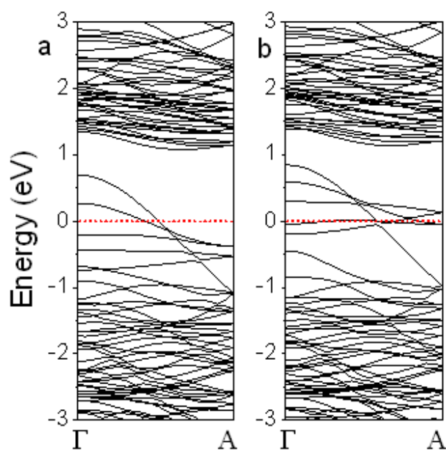
S-7, The calculated band structures of H-saturated zz-MoS 2 -NR-S-u: (a) spin-up and (b) spin-down.
