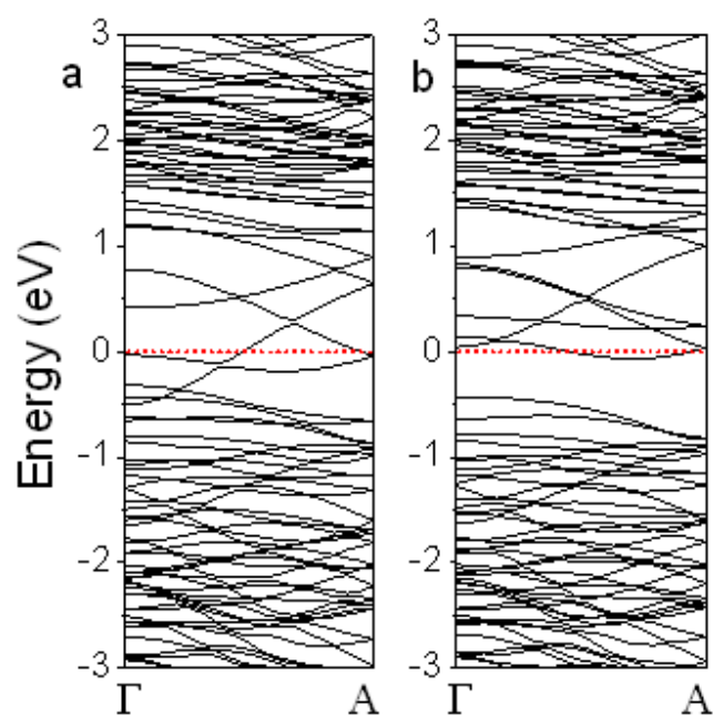
S-5, The calculated band structures of H-saturated zz\text{-MoS}_2\text{-NR-Mo-u} : (a) spin-up and (b) spin-down.
