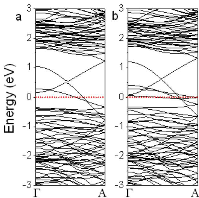
S-6, The calculated band structures of zz\text{-MoS}_2\text{-NR-S-u} : (a) spin-up and (b) spin-down.
