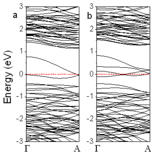
S-3, The calculated band structures of H-saturated zz-MoS 2 -NR-u: (a) spin-up and (b) spin-down.
