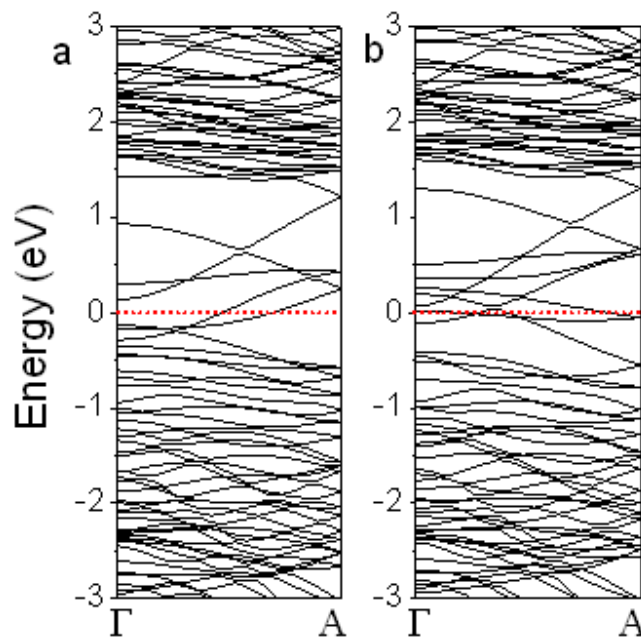
S-2, The calculated band structures of zz-MoS 2 -NR-u: (a) spin-up and (b) spin-down.
