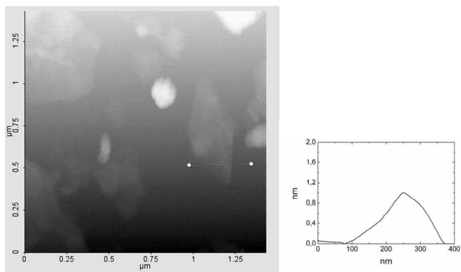
Figure S1: AFM image (left panel) and AFM height profile (right panel) of GO flakes.
