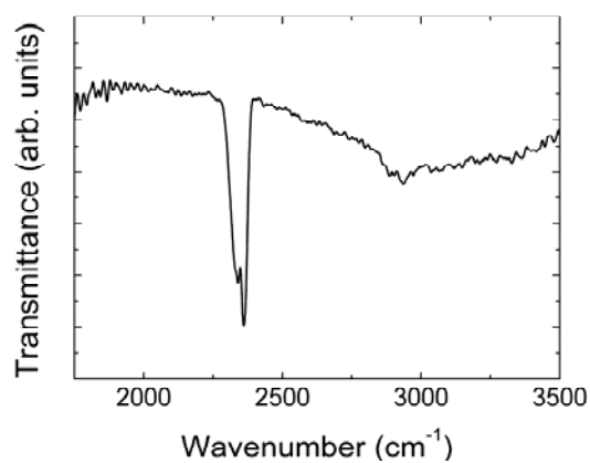
Figure S2: FTIR spectrum of APTES modified Si substrate.
