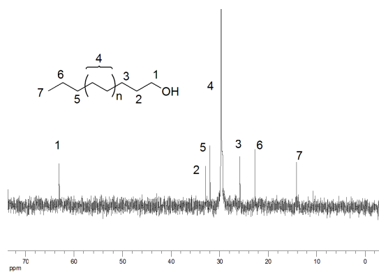
Figure S1. ^{13}\text{C} NMR spectrum of PE-OH in 1,2-dichlorobenzene- d_4 at 120 °C.
