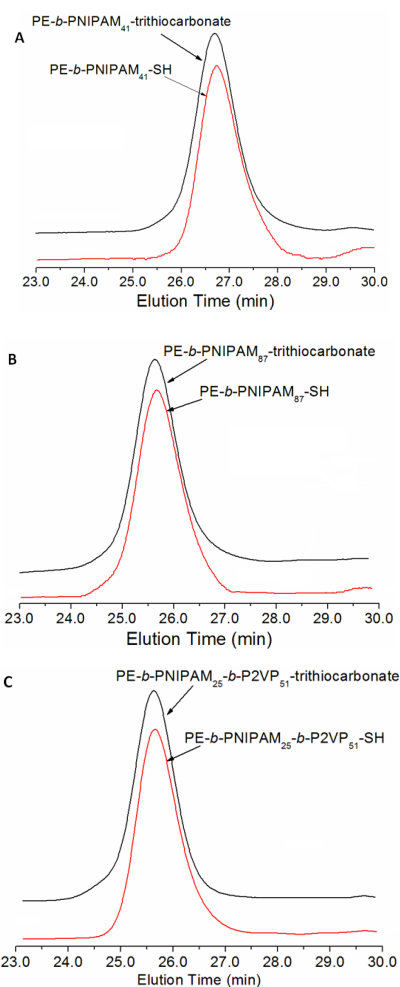
Figure S2. GPC traces of A PE- b -PNIPAM 41 B PE- b -PNIPAM 87 and C PE- b -PNIPAM 25 - b -P2VP 51
