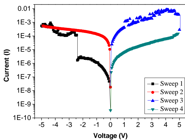
Fig. S3 Typical I–V characteristics of the ITO/ iamP7 (30 nm)/Al device.
