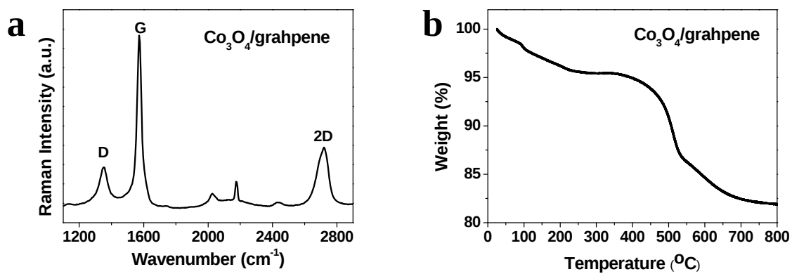
Figure S2. (a) Raman spectrum and (b) TGA results of \text{Co}_3\text{O}_4/\text{graphene} .
