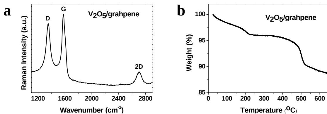
Figure S3. (a) Raman spectrum and (b) TGA results of V_2O_5 /graphene.
